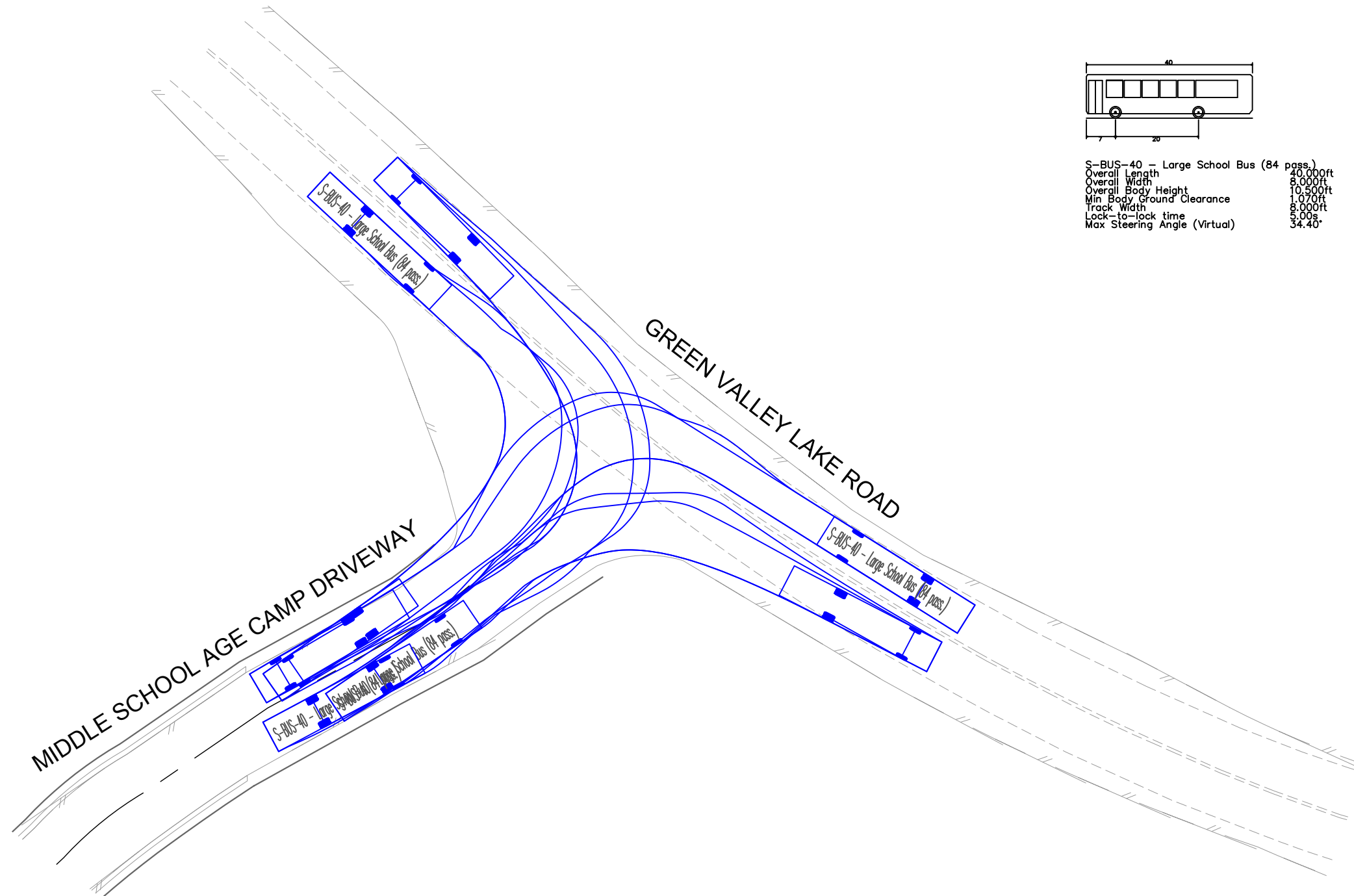
EXHIBIT 3 TRUCK TURNS - MIDDLE SCHOOL AGE CAMP DRIVEWAY
